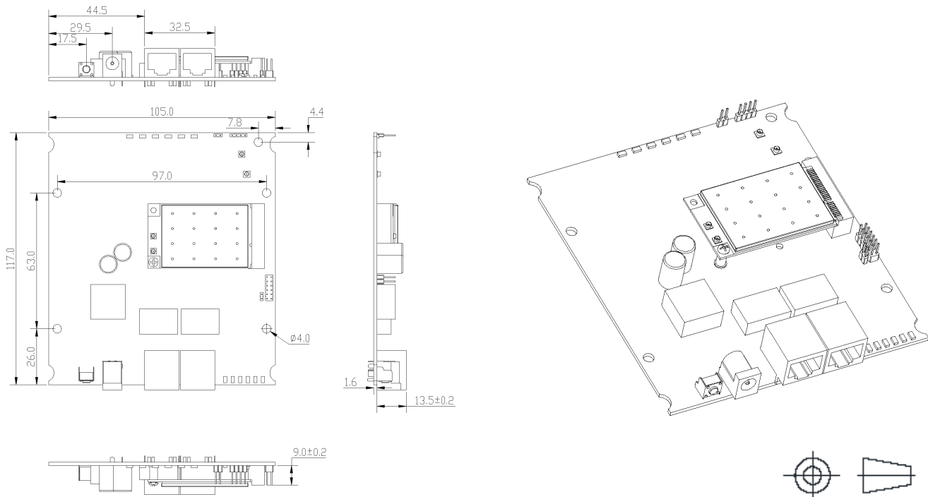
Dimensional Drawing of WPJ344 with WLE600VX (Normal Card Form Factor)
